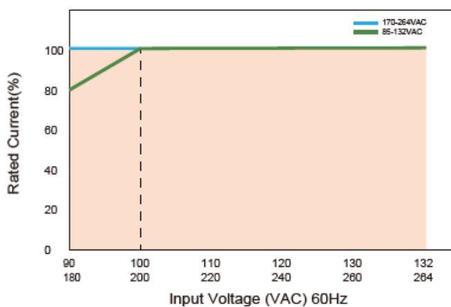
Static Characteristics
