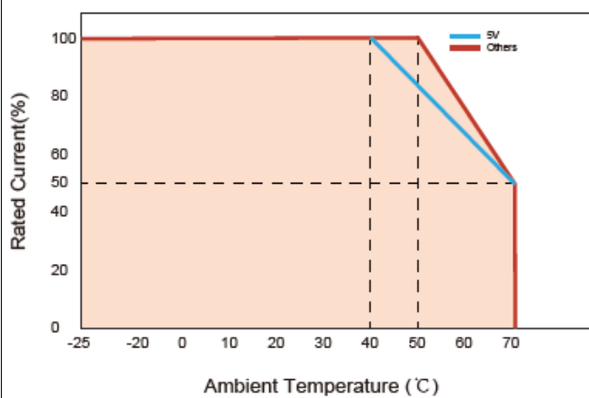
Derating Curve
